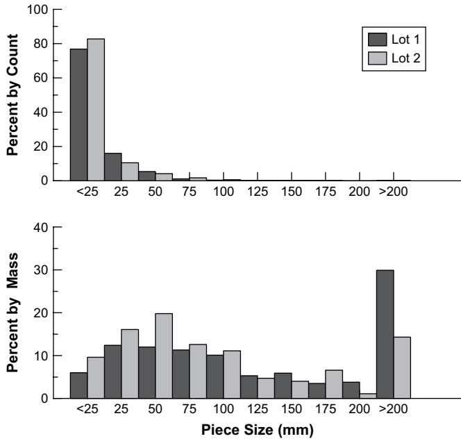
Fig. 1. Material characteristics based on percent by mass and percent by count from two lots of wood shreds. Lot 1 was used during the sandy loam soil testing and lot 2 was used during gravelly sand soil testing.
