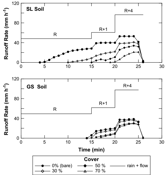
Fig. 3. Average runoff hydrographs for four coverage amounts of wood shreds on fine-grained sandy loam soil (SL) and coarse-grained gravelly sand (GS) soil.
