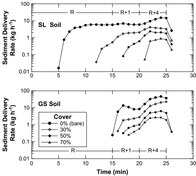
Fig. 4. Average sediment delivery rates for four coverage amounts of wood shreds on sandy loam (SL) and gravelly sand (GS) soil. Note the logarithmic scale for sediment delivery rate.
