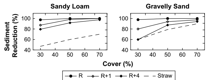
Fig. 5. Average sediment reduction compared to bare plot for three different coverage amounts of wood shreds and estimated sediment reduction for agricultural straw based on Burroughs and King (1989) for silt content and slope used in the present study.
