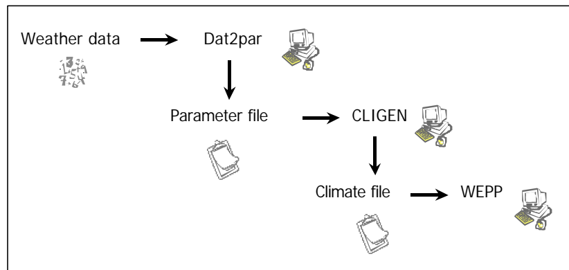
Figure 1: The CLIGEN data path
