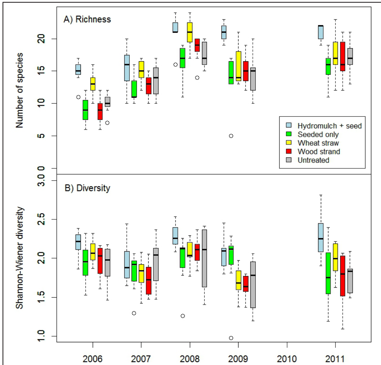
Figure 2. Species richness and diversity for four post-fire rehabilitation treatments and a similar but untreated area for 2006 through 2011 (we did not sample in 2010), one to six years after mulch treatments were applied in fall 2005 on the School Fire, Washington, USA. Data are shown as box plots with median and 25 th and 75 th percentiles. The same seven plots in each treatment were sampled each year.
