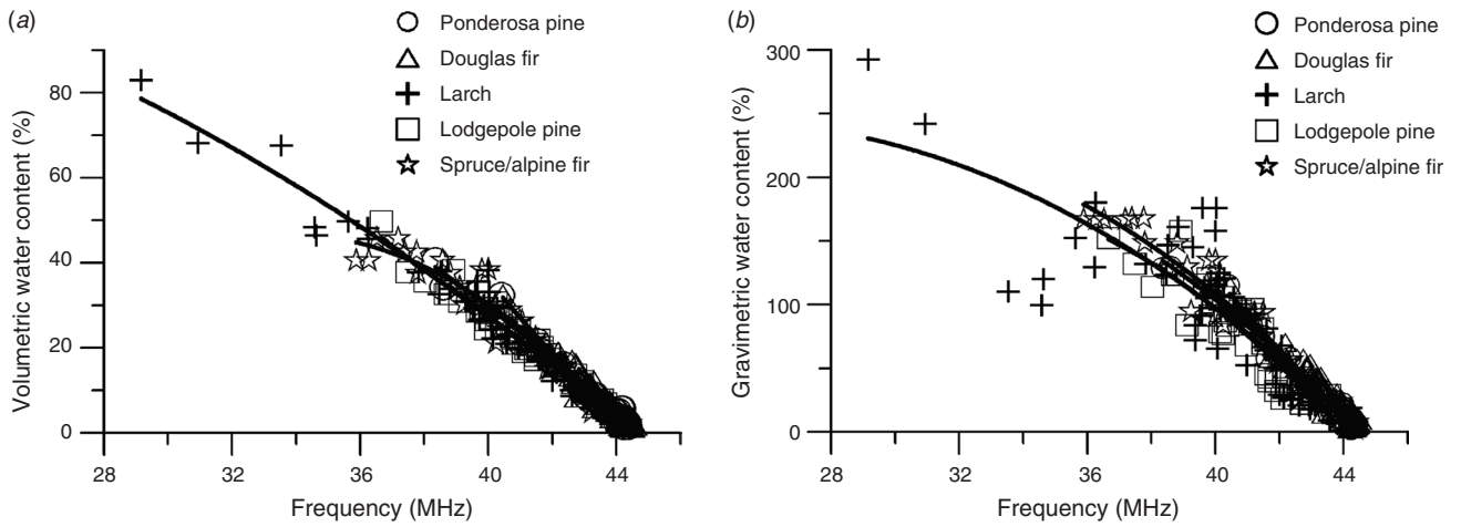
Fig. 6. The frequency readings taken at Bass Creek/Nine Mile Creek, Montana site were plotted against (a) the laboratory measured VWC and (b) the laboratory measured GWC. Best-fit curves for each cover type duff show the relationship of duff moisture meter frequency readings to VWC and GWC. The corresponding equations are listed in Table 1.
