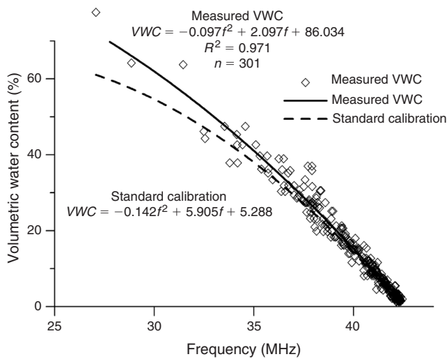
Fig. 11. Validation of the standard VWC calibration is graphically demonstrated by plotting the 1999 Bass Creek/Nine Mile Creek, Montana duff moisture meter measurements (adjusted for the factory-tuned CS615 circuit card) with the laboratory measured VWC for the samples.
