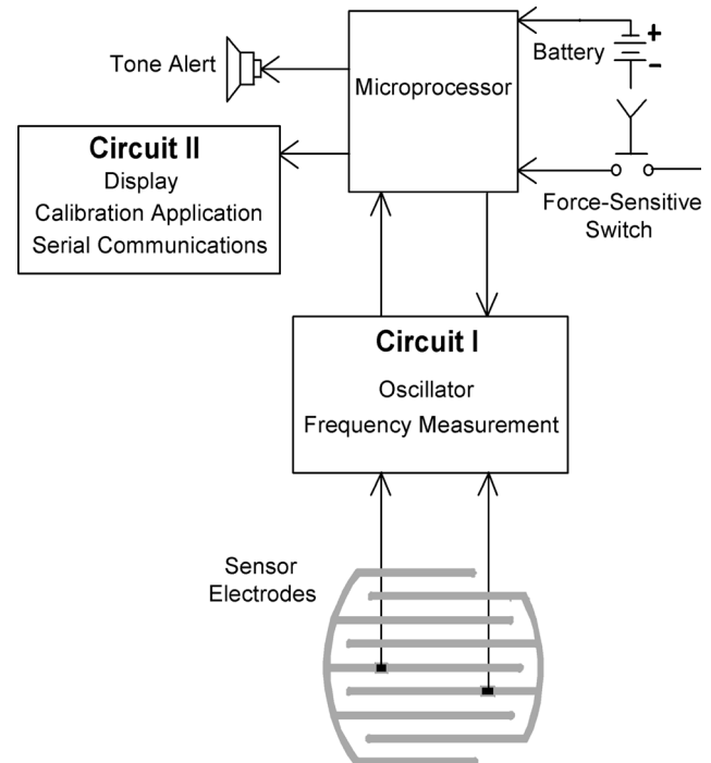
Fig. 3. Circuitry block diagram for the duff moisture meter.
