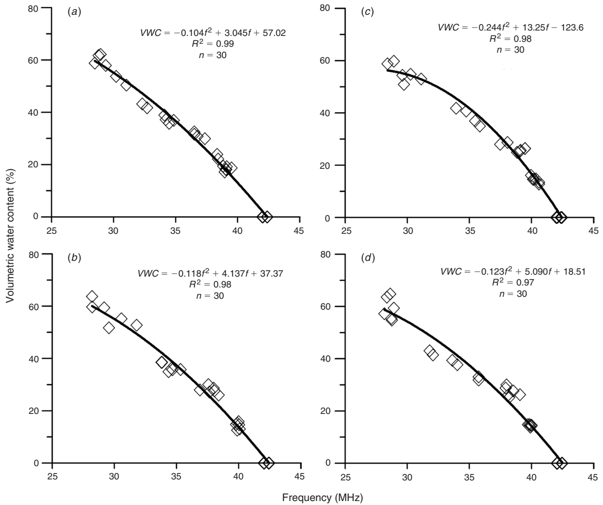
Fig. 7. The duff moisture meter VWC calibration curves were developed for four duff cover types: (a) Douglas fir, (b) larch, (c) lodgepole pine and (d) spruce/alpine fir. Six samples from each cover type at five moisture contents, including oven dry, were tested.
