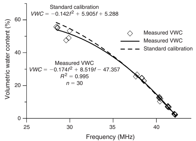
Fig. 10. Validation of the standard VWC calibration is graphically demonstrated by plotting the eastern hardwood duff moisture meter measurements with the laboratory measured VWC for the samples.
