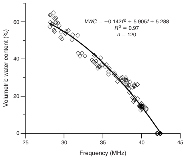
Fig. 8. The DMM600 standard calibration curve was derived from the combination of data from four duff cover types: Douglas fir, larch, lodgepole pine and spruce/alpine fir.
