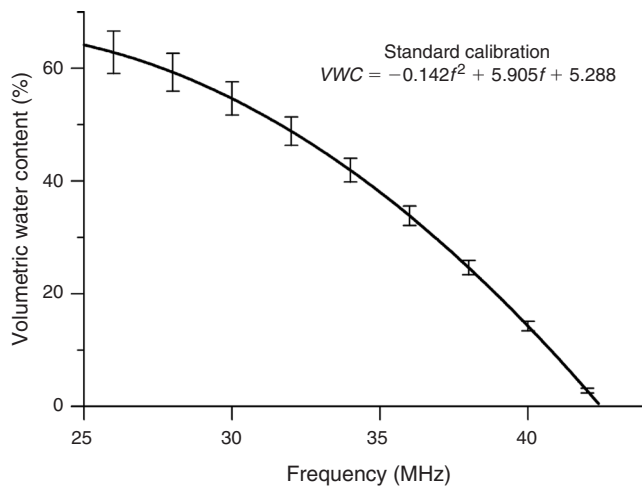
Fig. 9. The error bars on the standard calibration curve for the DMM600 duff moisture meter show that variations are smallest for lower volumetric water contents. After DMM600 Instruction Manual 2002 (Campbell Scientific, Inc. 2002).
