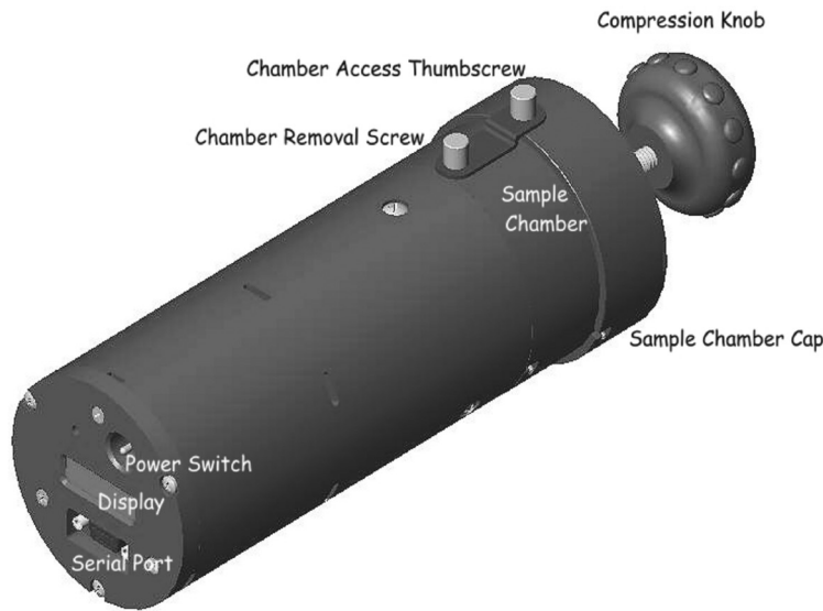
Fig. 1. DMM600 duff moisture meter (Campbell Scientific, Inc., Logan, UT).
