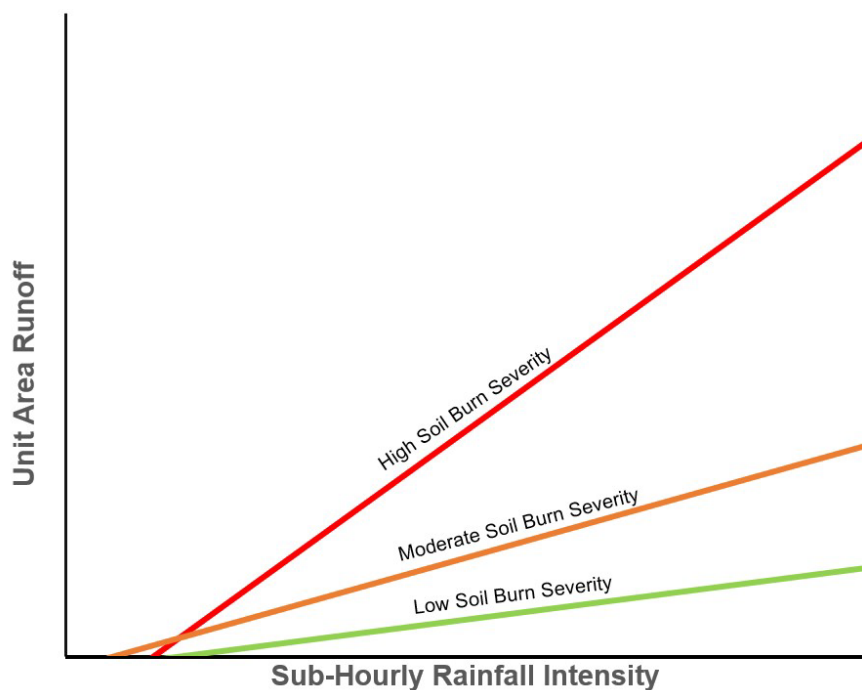
Figure 11. Peak stream flow rates in areas of different soil burn severities in the northern part of the California Coast Ranges. Lines reflect the difference in the runoff and rainfall intensity relationship among catchments burned at different soil burn severities for the first winter (2015-2016) following the 2015 Valley Fire at Boggs Mountain Demonstration State Forest.
